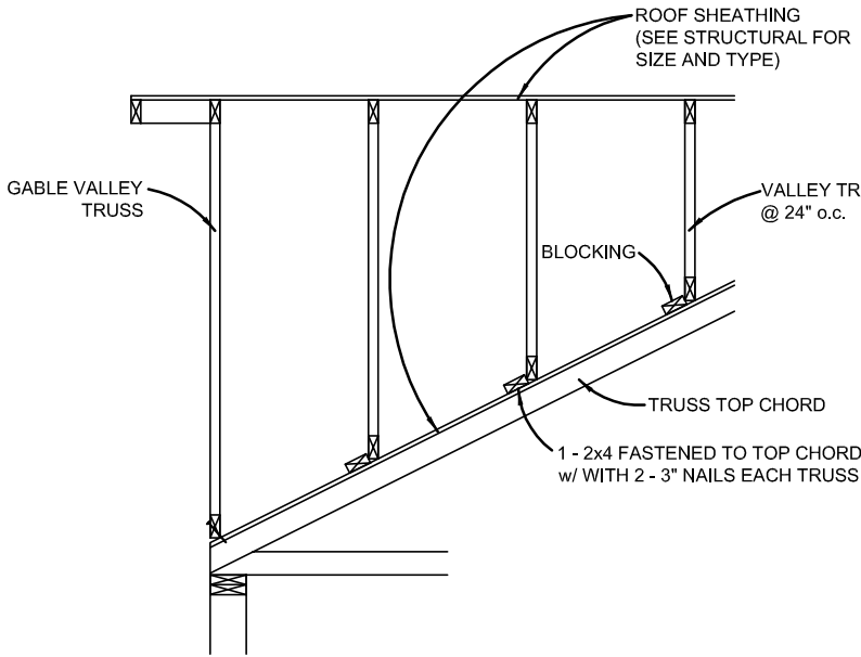
VALLEY AT GABLE END
