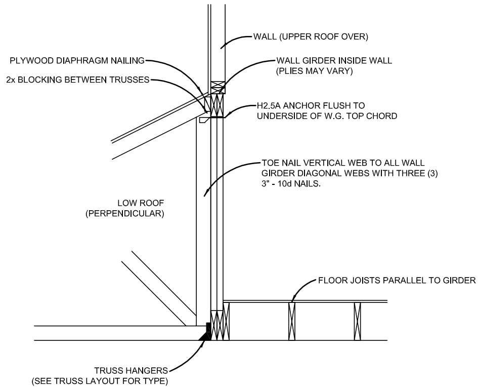
D WALL GIRDER INSIDE, ROOF PERPENDICULAR, FLOOR PARALLEL NOT TO SCALE
