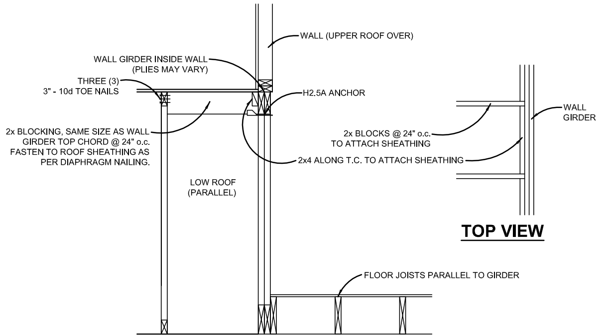
C WALL GIRDER INSIDE, ROOF PARALLEL, FLOOR PARALLEL NOT TO SCALE
