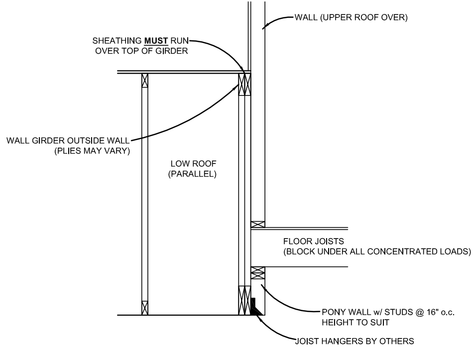
J WALL GIRDER OUTSIDE, ROOF PARALLEL WITH PONY WALL NOT TO SCALE
