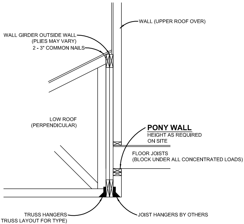
K WALL GIRDER OUTSIDE, ROOF PERPENDICULAR WITH PONY WALL NOT TO SCALE
