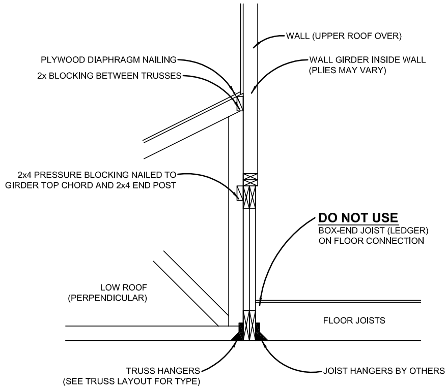
P WALL GIRDER INSIDE, ROOF PERPENDICULAR, FLOOR PERPENDICULAR NOT TO SCALE
