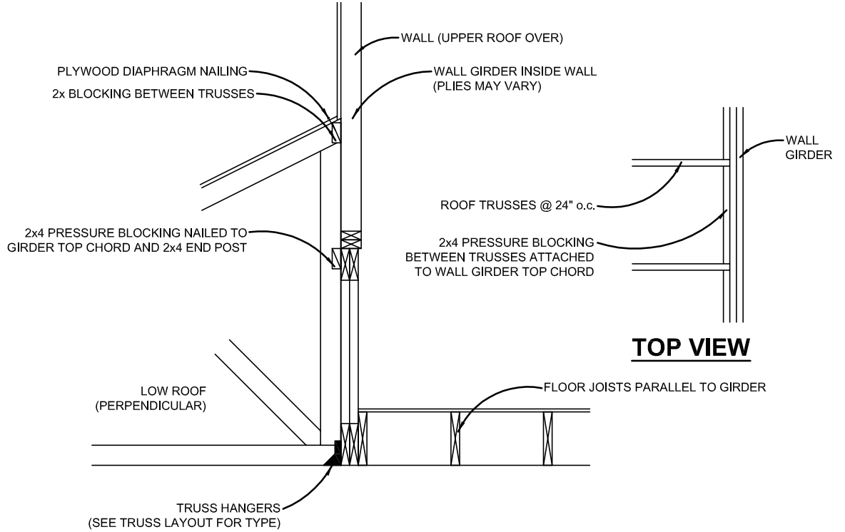
N WALL GIRDER INSIDE, ROOF PERPENDICULAR, FLOOR PARALLEL NOT TO SCALE
