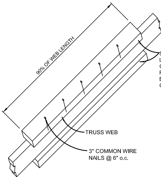
I-BRACE DETAIL
