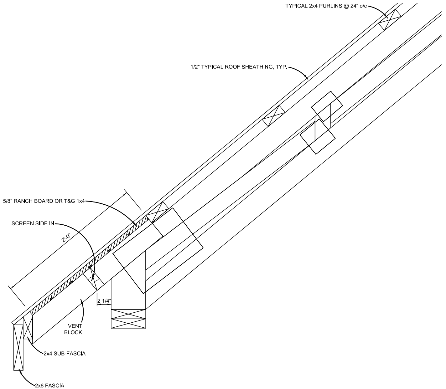
TYPICAL OVERHANG DETAIL NOT TO SCALE
